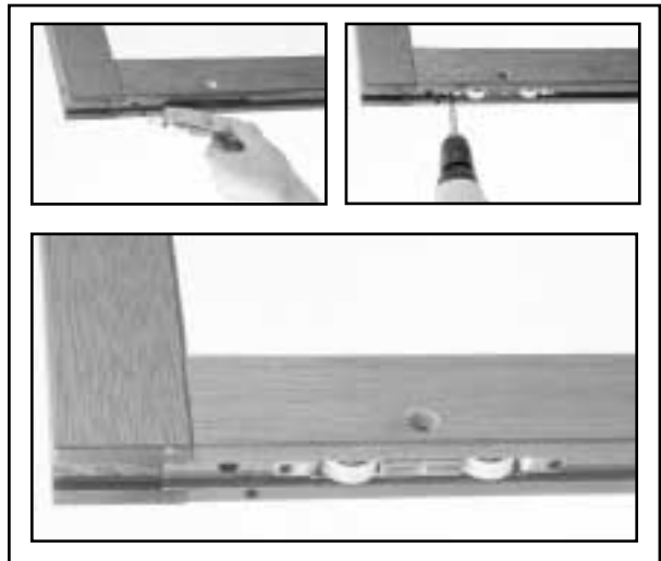
20 Fitting rollers to sliding door.
