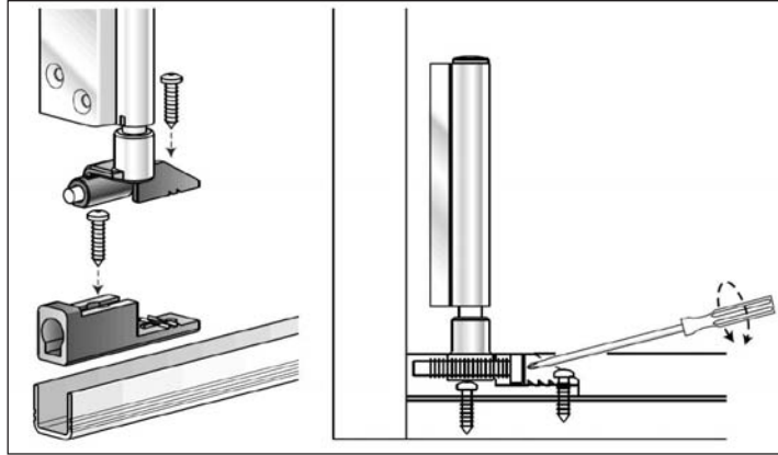
Fig. 13: Fixing and adjusting the bottom pivot blocks
